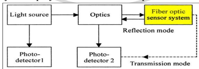
Fig. 2. Block diagram of a generic optical fiber sensor
