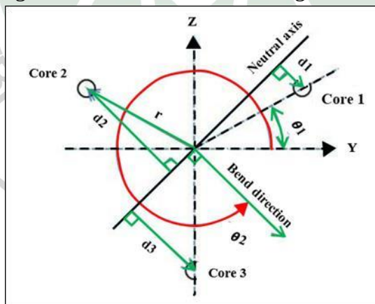
Fig. 3. Circuit for the stress resulting from bending
